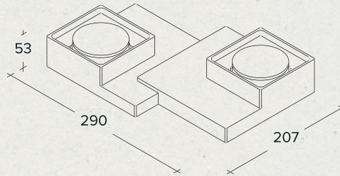
Two-lights plaster ceiling lamp (Modello depositato)
