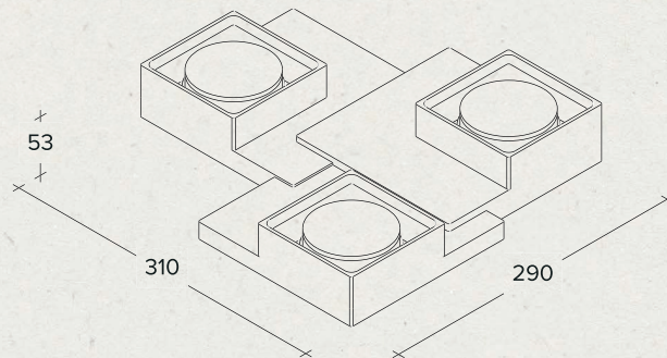
Three-lights plaster ceiling lamp (Modello depositato)
