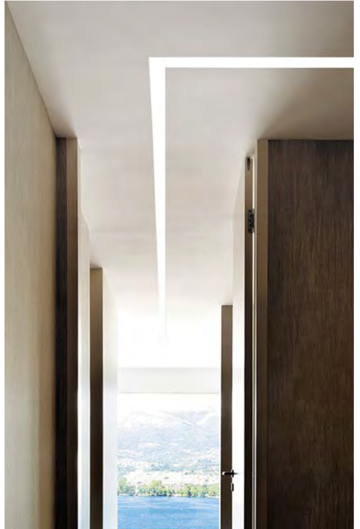
↑ T139 Eubea Extruded aluminium system with satin-finished cover w35,2 x h34,9 mm length: 500/1000/1500/2000 mm
