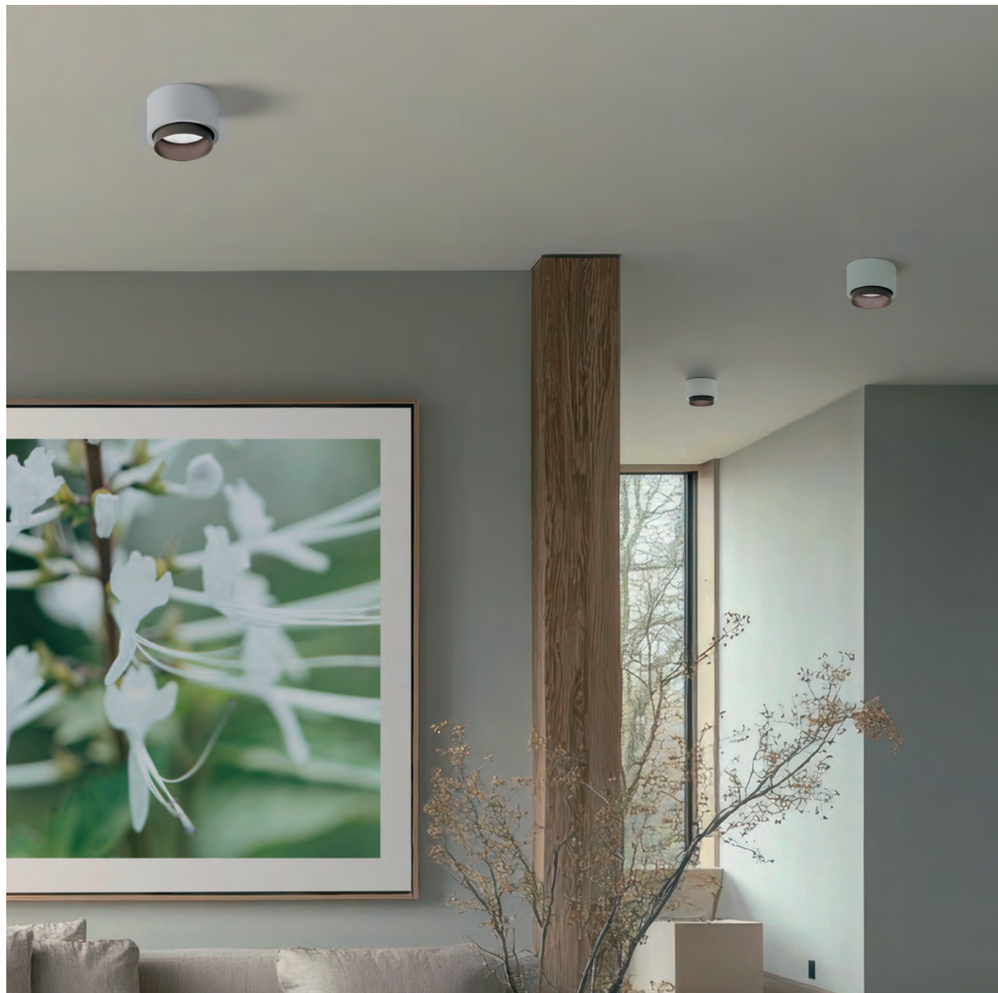
↑ → T497 Syme tonda Plaster ceiling lamp with satin bronze ring finishing GX53 – 1x10W Ø110 x h80 mm
