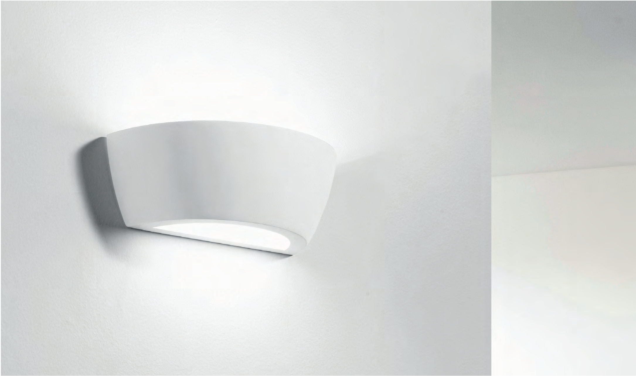
T106 Mantinea Up/Down plaster wall light E27 – 1x40W w250 x d130 x h90 mm
