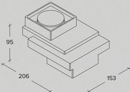
Two-lights Up/Down plaster wall lamp
