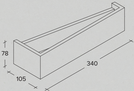
Up/Down plaster wall lamp
