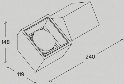
Plaster wall lamp with aluminium frames in different finishes
