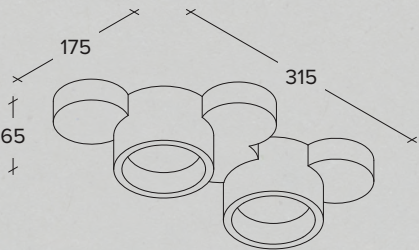
Two-lights plaster ceiling lamp (Modello depositato)
