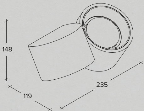
Plaster wall lamp with aluminium rings in different finishes
