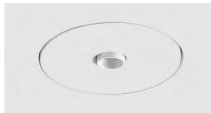
← ↑ T469 / T484* Rhodia Inspectable Recessed plaster spotlight with matte white painted ring finishing LED Module – 10,5W Ø20 mm aluminium ring
