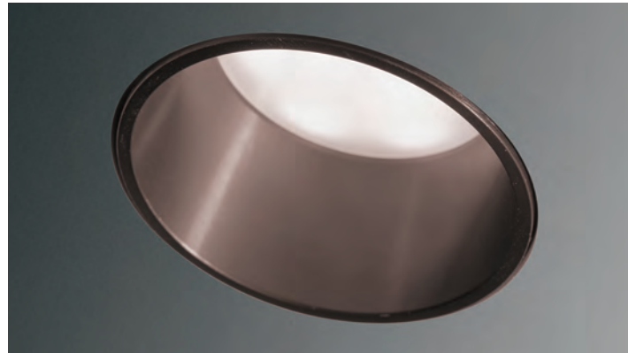
← ↓ T411 Thessaly Raso Flush recessed plaster spotlight with brushed bronze ring finishing GU10 - 1x10W Ø60 mm aluminium ring
