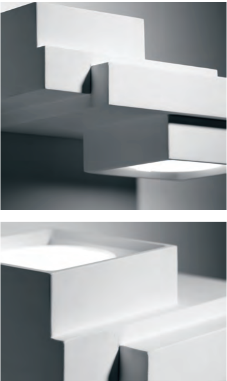
← ← ↓ T380 Sibari Two-lights Up/Down plaster wall lamp GX53 – 2x10W w206 x d153 x h95 mm Technical data 503
