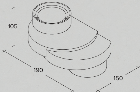
Up/Down two-lights plaster wall lamp (Modello depositato)
