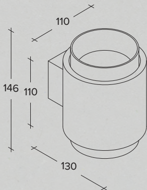
Plaster wall lamp for indirect lighting with aluminium rings in different finishes
