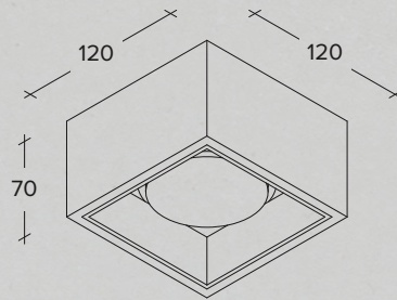
Plaster ceiling lamp with aluminium frame in different finishes
