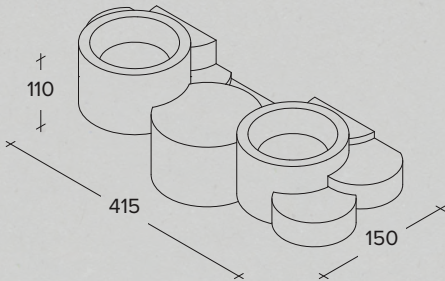
Up/Down three-lights plaster wall lamp (Modello depositato)
