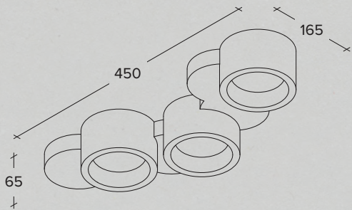
Three-lights plaster ceiling lamp (Modello depositato)
