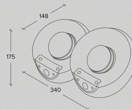
Plaster wall lamp for indirect lighting (Modello depositato)
