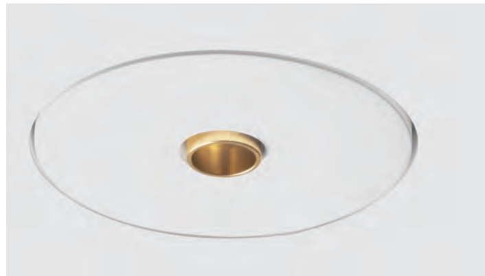
↓ → T470 / T485* Rhodia Inspectable Recessed plaster spotlight with satin brass ring finishing LED Module – 10,5W Ø20 mm aluminium ring
