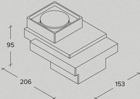
Up/Down two-lights plaster wall lamp
