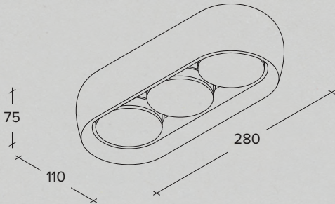
Three-lights plaster ceiling lamp Quartz Grey (RAL 7039)
