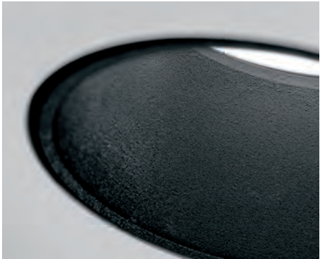
↓→→ T390 Thessaly Raso Flush recessed plaster spotlight with matte black painted ring finishing GU10 – 1x10W Ø60 mm aluminium ring Technical data 441
