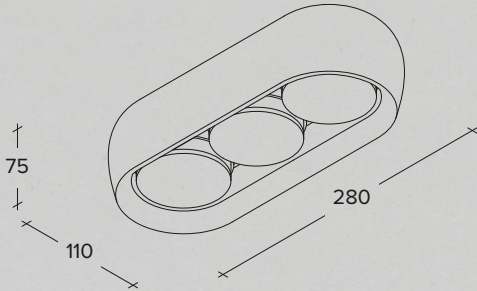
Three-lights plaster ceiling lamp white
