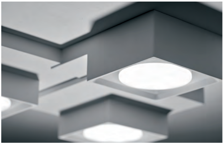
↑ ↑ T378 Sibari Three-lights plaster ceiling lamp GX53 – 3x10W w310 x d290 x h53 mm Technical data 502
