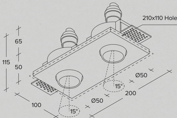
Two-lights adjustable recessed plasterboard spotlight with matte black painted rings finishing. Adjustable 15° tilt light
