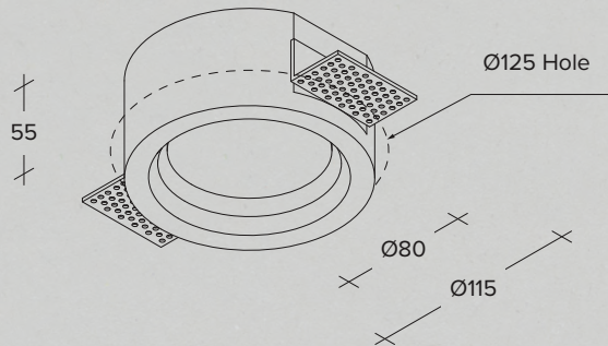
Recessed plaster spotlight
