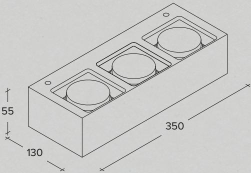
Three-lights plaster wall lamp
