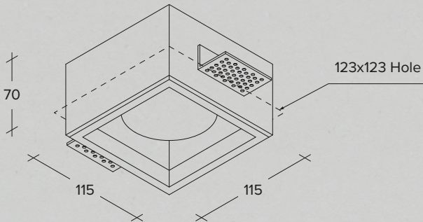
Recessed plaster spotlight
