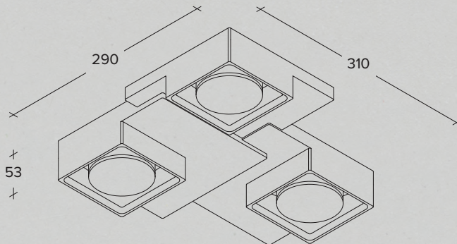
Three-lights plaster ceiling lamp (Modello depositato)
