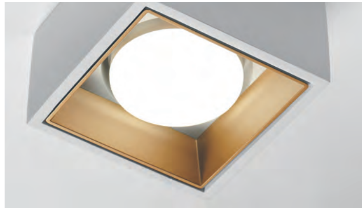
↓ → T428 Nasso quadrata Plaster ceiling lamp with satin brass frame finishing GX53 – 1x10W w120 x d120 x h70 mm
