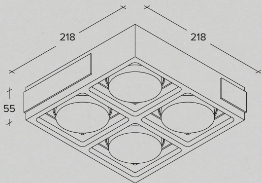
Plaster ceiling lamp with aluminium elements in different finishes
