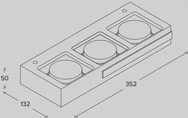
Plaster wall lamp with aluminium element in different finishes
