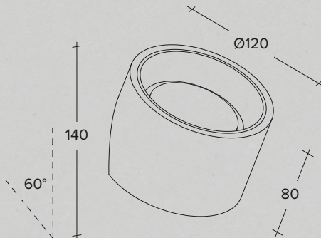
Plaster wall lamp with aluminium ring in different finishes
