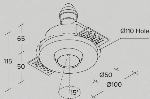
One-light adjustable recessed plasterboard spotlight with matte black painted ring finishing. Adjustable 15° tilt light
