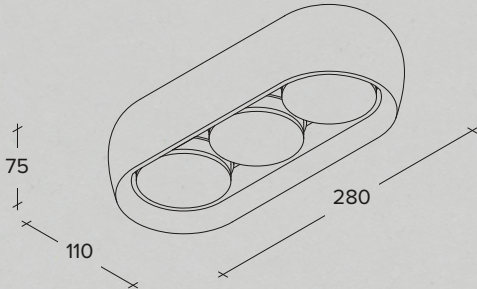
Three-lights plaster ceiling lamp white
