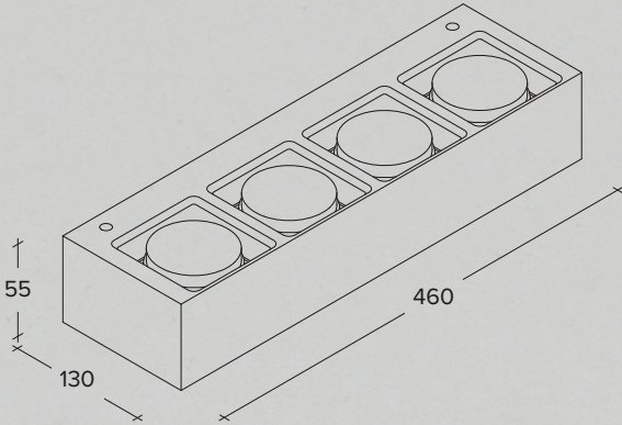
Four-lights plaster wall lamp
