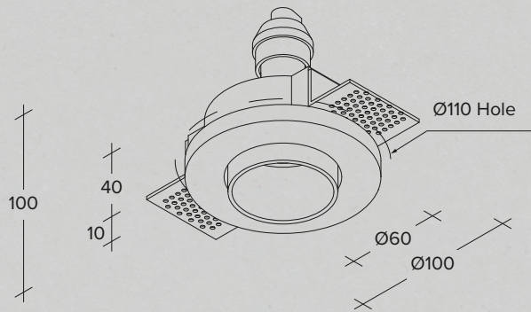
Recessed plaster spotlight with aluminium ring
