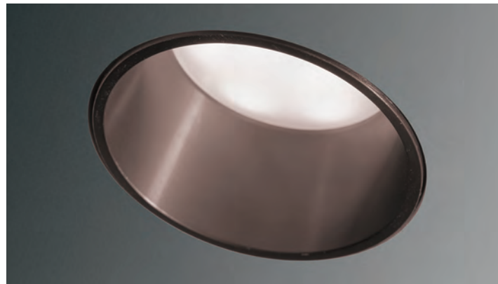
T411 Thessaly Raso Flush recessed plaster spotlight with brushed bronze ring finishing GU10 - 1x10W Ø60 mm aluminium ring
