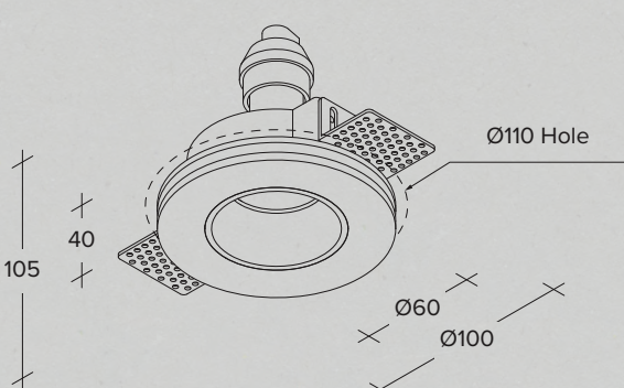
Flush recessed plaster spotlight with aluminium ring
