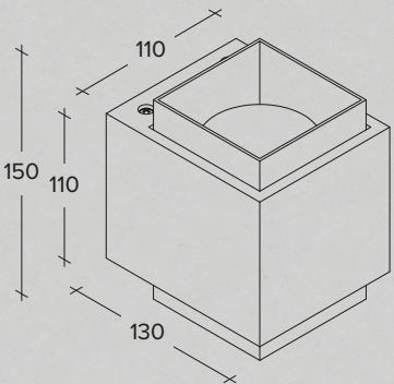
Up/Down plaster wall lamp with aluminium frames in different finishes
