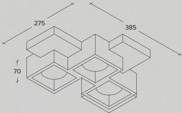
Three-lights plaster ceiling lamp
