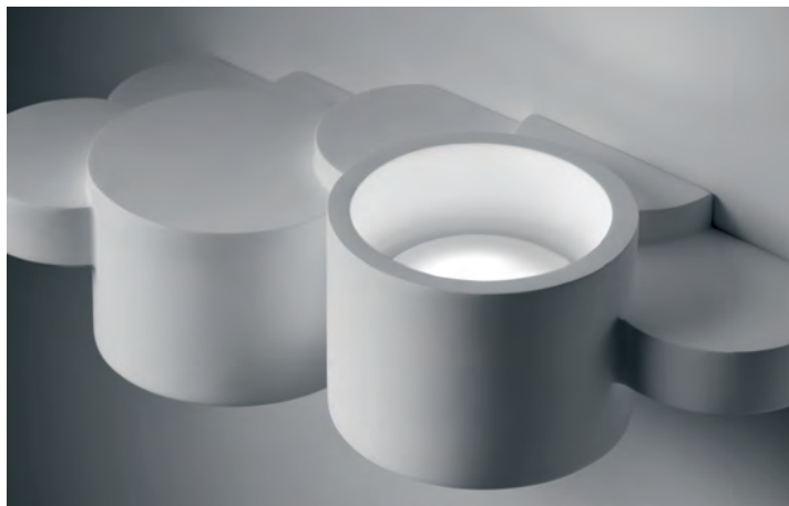
↓ → T321 Chio Up/Down two-lights plaster wall lamp GX53 – 2x10W w340 x d150 x h105 mm
