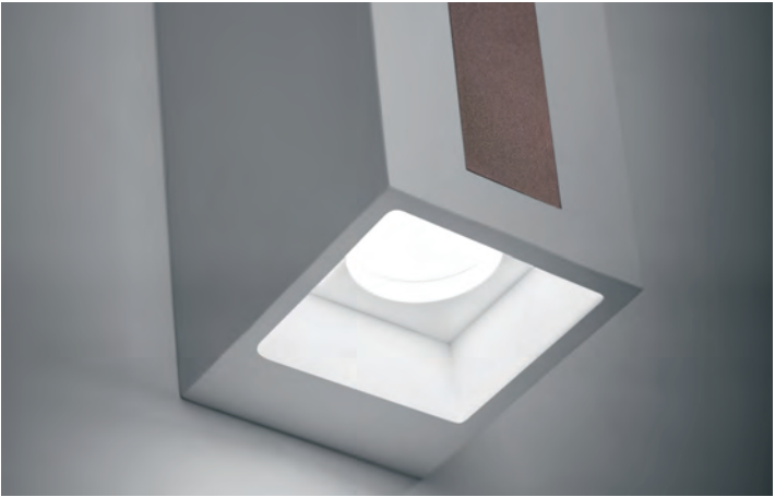
↓ → → T580 Thera Up/Down plaster wall lamp for indirect lighting with satin bronze painted element GU10 – 2x10W w80 x d97 x h205 mm
