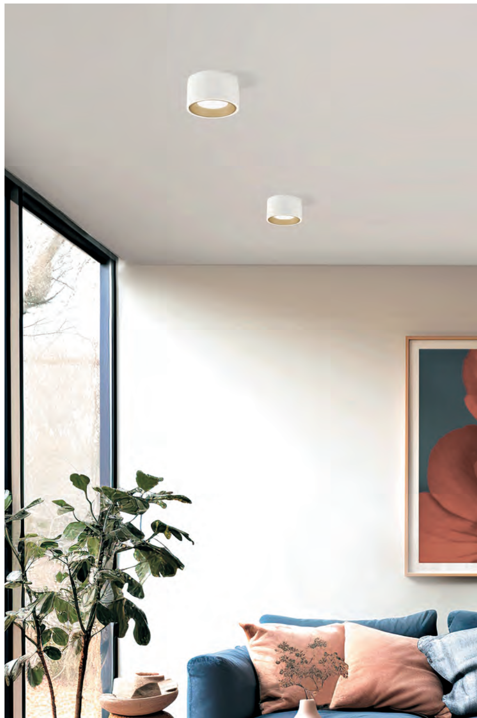
↓ → T424 Nasso tonda Plaster ceiling lamp with satin brass ring finishing GX53 – 1x10W Ø120 x h70 mm
