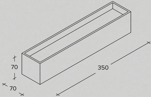
Up/Down plaster wall lamp
