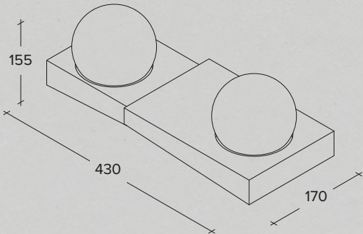
Plaster wall lamp with round blown glass (Modello depositato)
