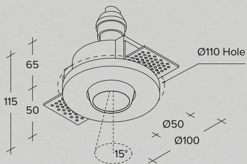
One-light adjustable recessed plasterboard spotlight with matte white painted ring finishing. Adjustable 15° tilt light
