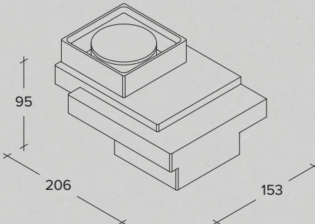
Up/Down two-lights plaster wall lamp
