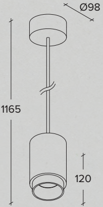
Plaster pendant lamp with aluminium rings in different finishes
