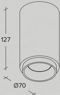
Plaster ceiling lamp with aluminium rings in different finishes
