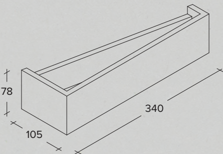
Up/Down plaster wall lamp
