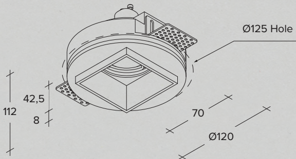
Recessed plaster spotlight with aluminium frame
