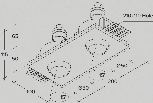
Two-lights adjustable recessed plasterboard spotlight with matte white painted rings finishing. Adjustable 15° tilt light
