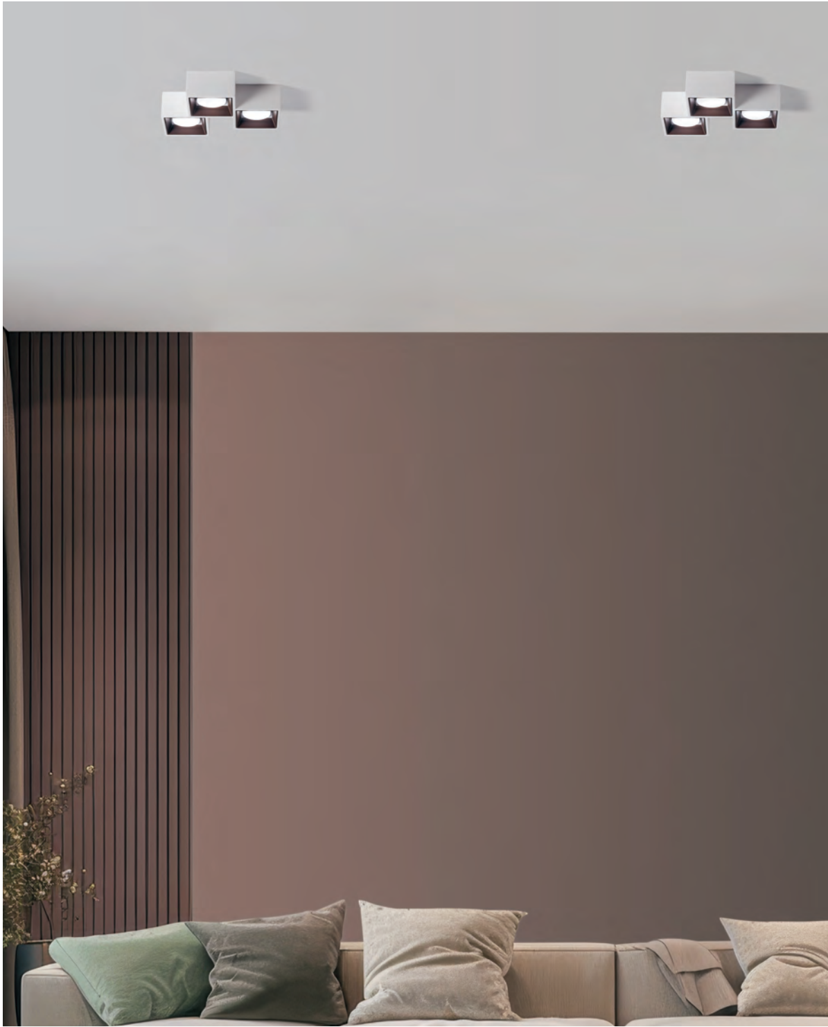
↓ → T515 Nasso quadrata Plaster ceiling lamp with satin bronze frames finishing GX53 – 3x10W w233 x d303 x h70 mm
