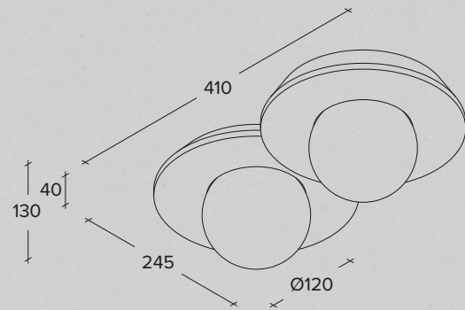
Plaster ceiling/wall lamp with round blown glass (Modello depositato)
