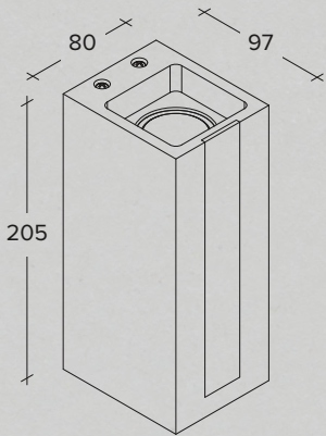
Up/Down plaster wall lamp with aluminium element in different finishes
