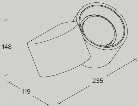
Up/Down plaster wall lamp with aluminium rings in different finishes
