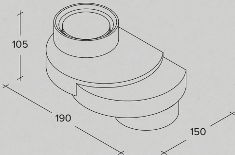
Up/Down two-lights plaster wall lamp (Modello depositato)
