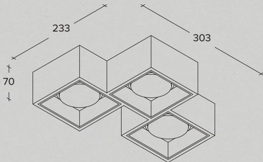
Plaster ceiling lamp with aluminium frames in different finishes
