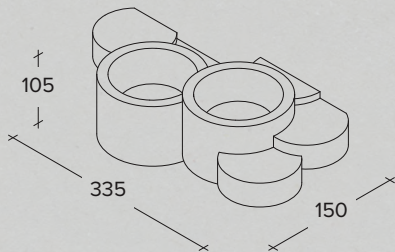
Two-lights plaster wall lamp (Modello depositato)
