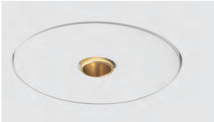
↓ → T470 / T485* Rhodia Inspectable Recessed plaster spotlight with satin brass ring finishing LED Module – 10,5W Ø20 mm aluminium ring Technical data 445
