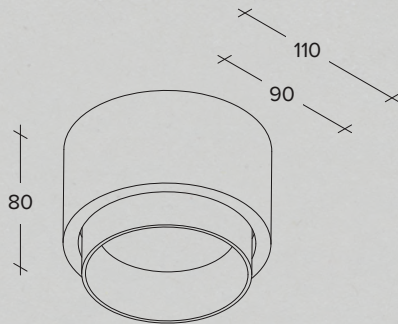
Plaster ceiling lamp with aluminium ring in different finishes
