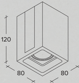
Plaster ceiling lamp with aluminium elements in different finishes
