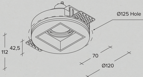
Flush recessed plaster spotlight with aluminium frame
