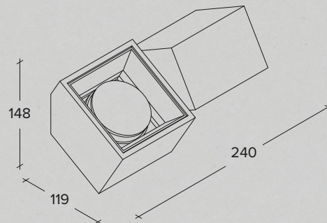
Up/Down plaster wall lamp with aluminium frames in different finishes
