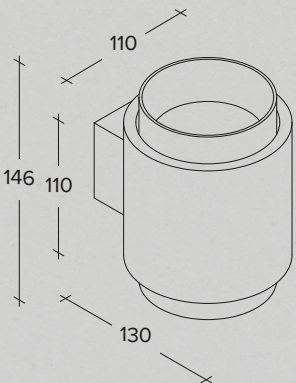
Up/Down plaster wall lamp for indirect lighting with aluminium rings in different finishes
