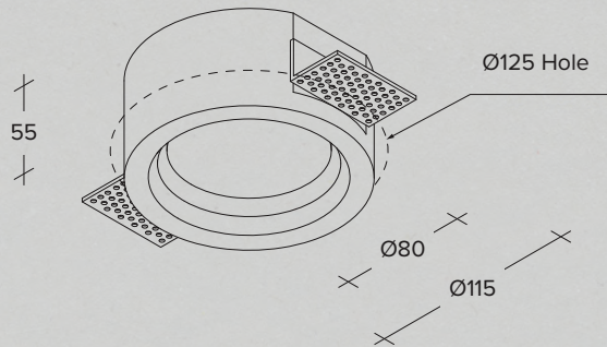
Recessed plaster spotlight with black painted inner edge
