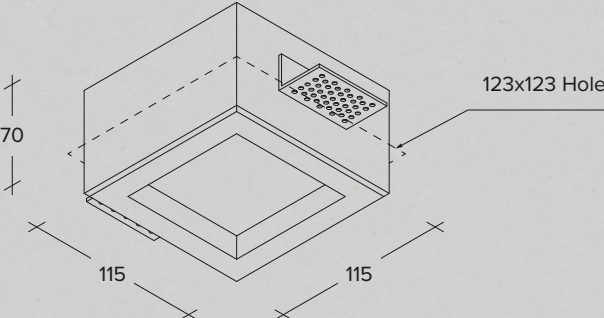
Recessed plaster spotlight with black painted inner edge and opal glass
