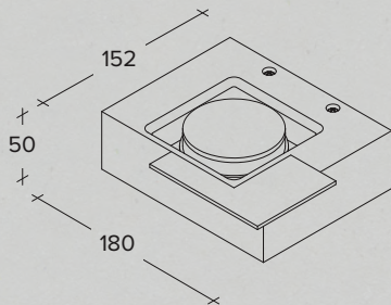
Plaster wall lamp with Quartz Grey (RAL 7039) painted aluminium element
