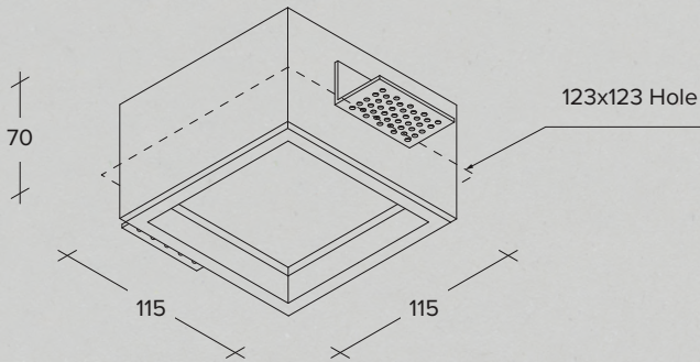
Recessed plaster spotlight with opal glass
