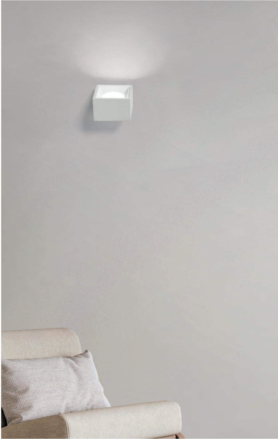
↓ → T435 Nasso quadrata Plaster wall lamp for indirect lighting with matte white painted frame finishing GX53 – 1x10W w120 x d120 x h140 mm Technical data 475
