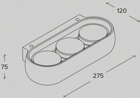
Three-lights plaster wall lamp white
