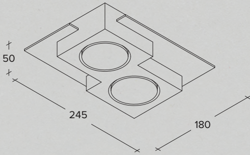
Plaster ceiling lamp with Quartz Grey (RAL 7039) painted aluminium elements
