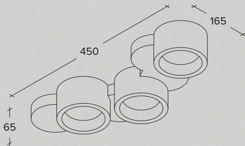
Three-lights plaster ceiling lamp (Modello depositato)
